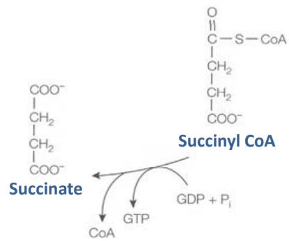
Succinate thiokinase
