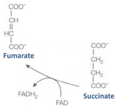
Succinate dehydrogenase
